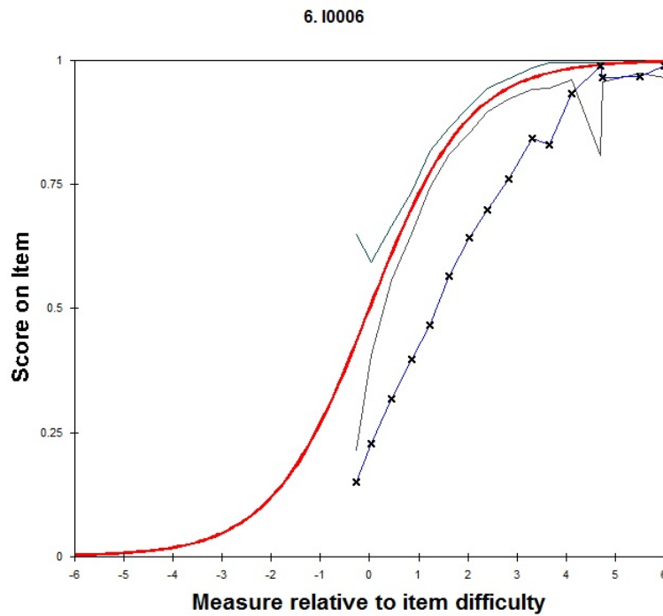
Figure 4.28 Empirical Conditional Mean Scores and Expected Response Function Item 6.
