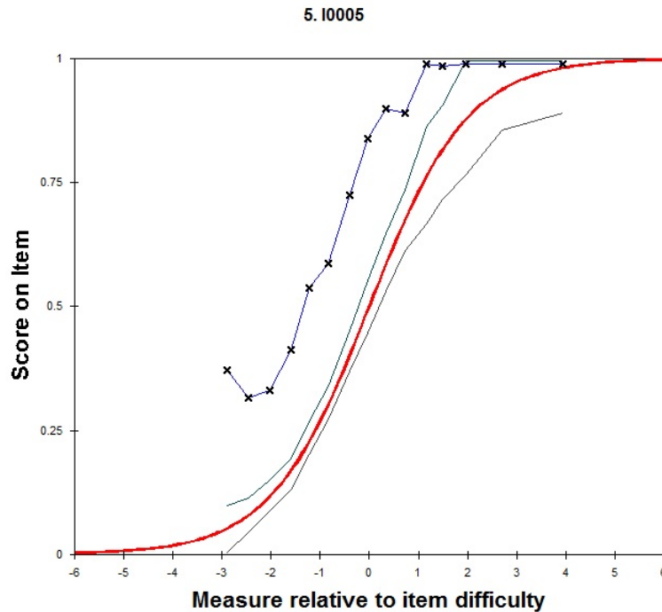
Figure 4.27 Empirical Conditional Mean Scores and Expected Response Function Item 5.
